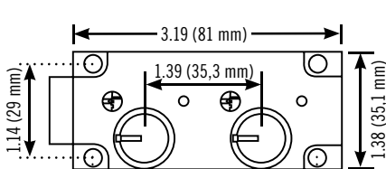
4420—designed for matchwork to all Corbin guard keys (RH model shown here)
